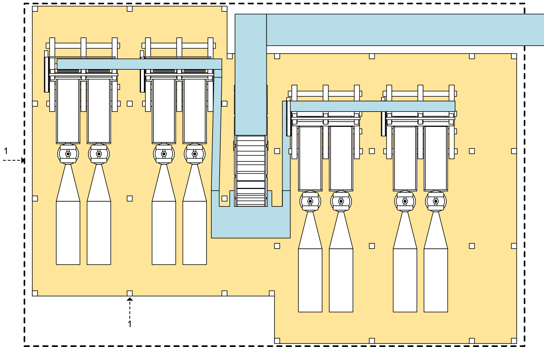
Kimber Mill – Floor Plan Scale: 3/32" = 1 ft
