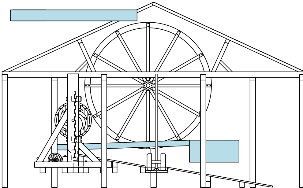
West View #1
