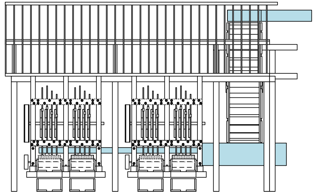
North View #1
